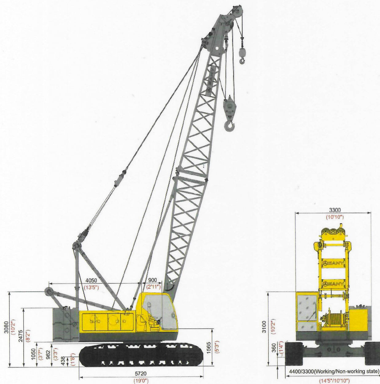
Outline Dimensions of SCC500E Hydraulic Crawler Crane
