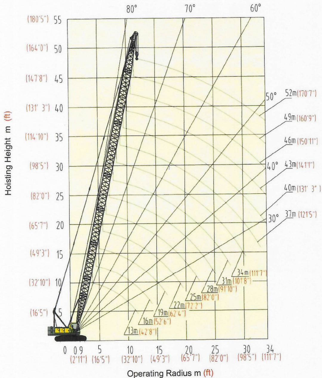
Main Boom Hoisting Height Diagram
