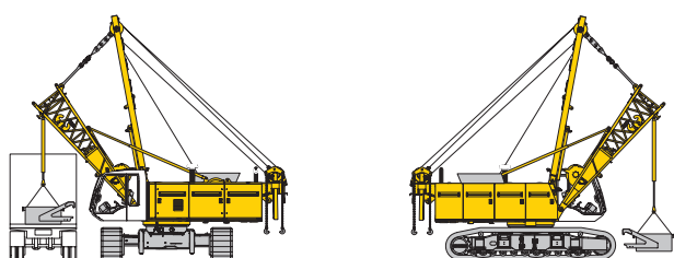
Unloading and assembly of carbody counterweight
