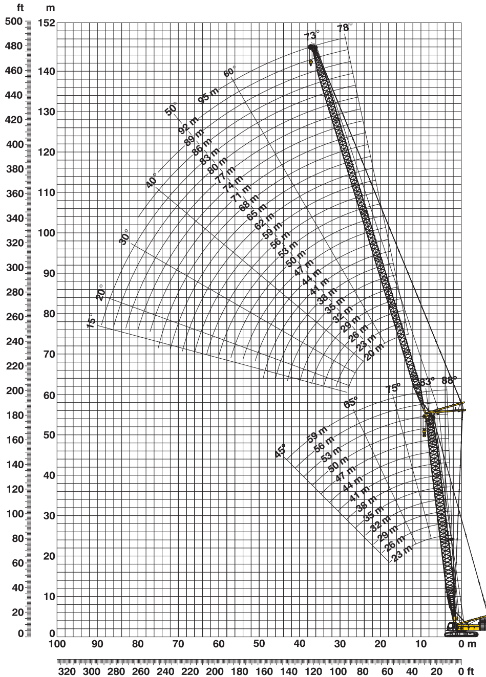
Boom configuration for main boom lengths (23 m – 59 m) (see table 1 on page 10)
